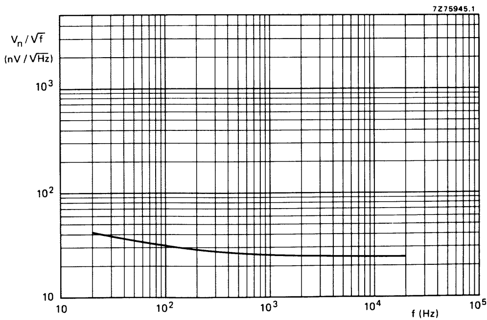
Fig.3 Equivalent input noise voltage.
